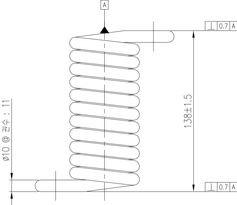
TORQUE 15,484kgf-mm(FORCE 75.0kgf) @ 30^\circ \pm 5^\circ TURN
