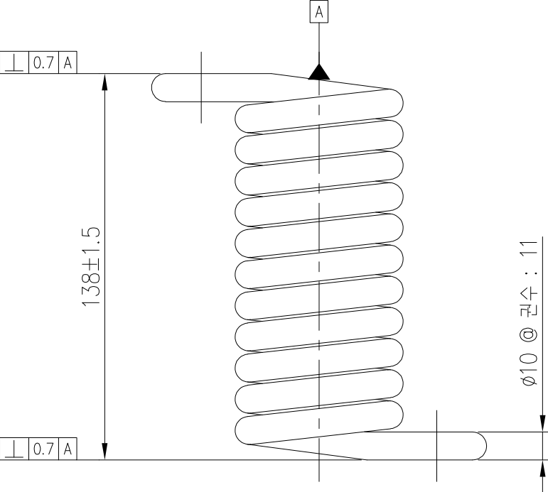
TORQUE 15,484kgf-mm(FORCE 75.0kgf) @ 30^\circ \pm 5^\circ TURN
