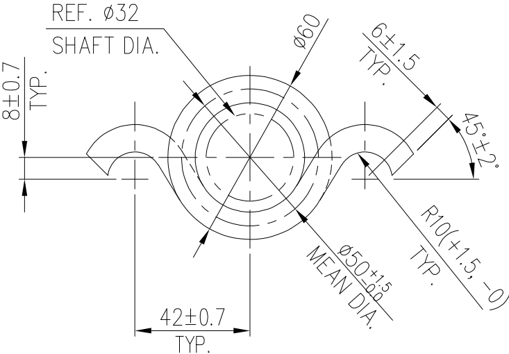
TORQUE 15,484kgf-mm(FORCE 75.0kgf) @ 30^\circ \pm 5^\circ TURN
